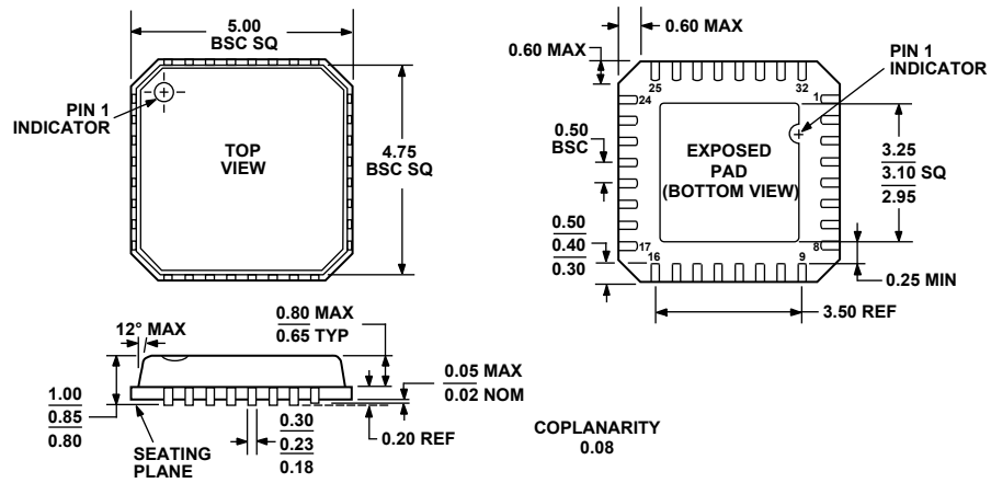
COMPLIANT TO JEDEC STANDARDS MO-220-VHHD-2 Figure 17. 32-Lead Lead Frame Chip Scale Package [LFCSP_VQ] 5 mm x 5 mm Body, Very Thin Quad (CP-32-2) Dimensions shown in millimeters
